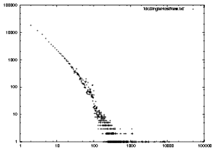
Figure 5.2. In-degree distribution of the crawled host graph. Multiple links between sites were treated as single. X-axis: value of in-degree, Y-axis: number of nodes having that in-degree
